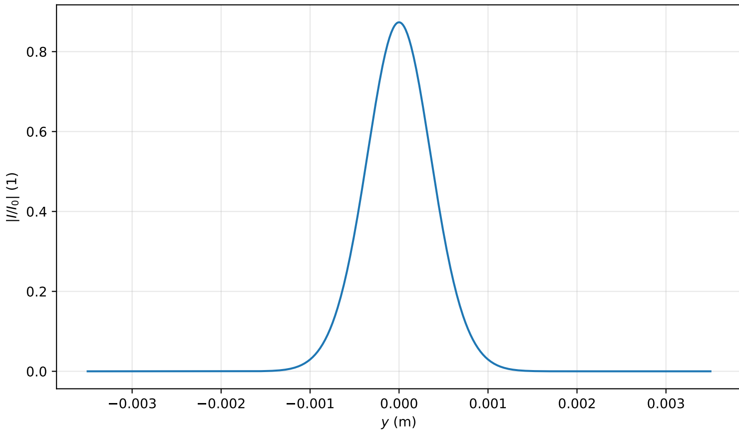
Intensity profile I(x=0, y, z=1.035)/I_0 , P_{in}=0.2P_{cr} , artificial time
